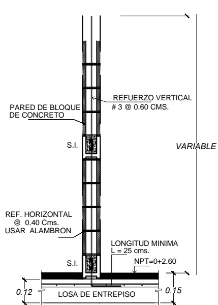
AMARRE DE PARED A LOSA
