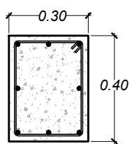
COLUMNA C-1
