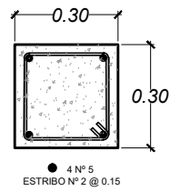
TENSOR T-1
