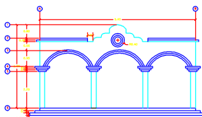
ELEVACION PRINCIPAL PORTAL COLONIAL
