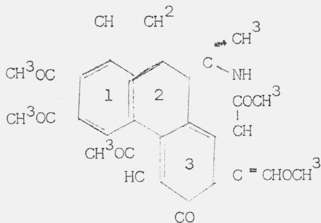
De-acetyl-methyl-colchicine
